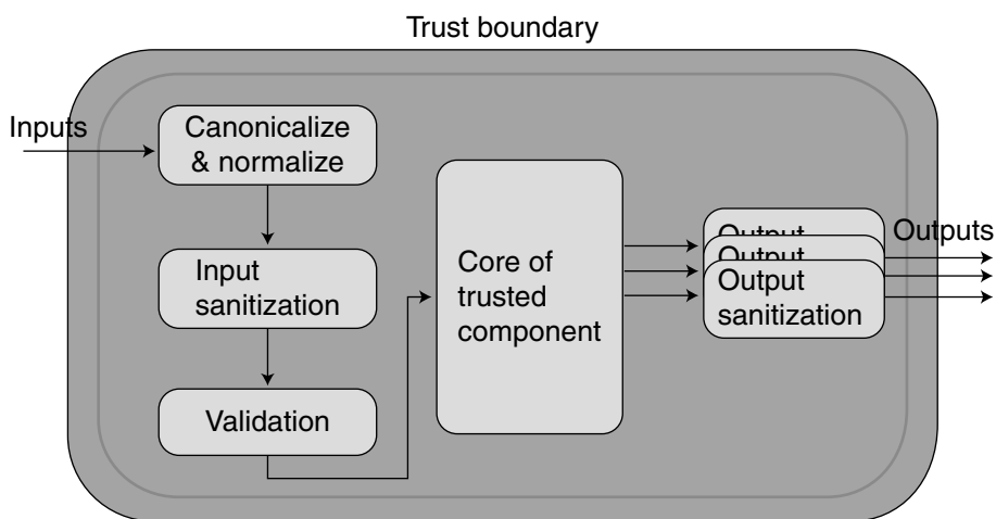
Figure 9.7 Trusted component
