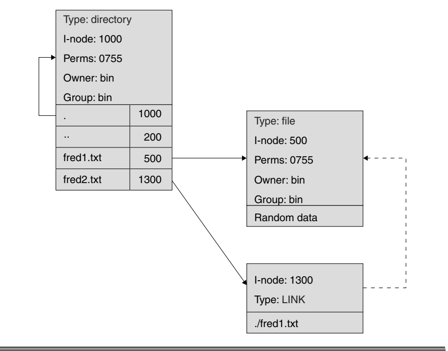
Figure 8.9 Symbolic link
