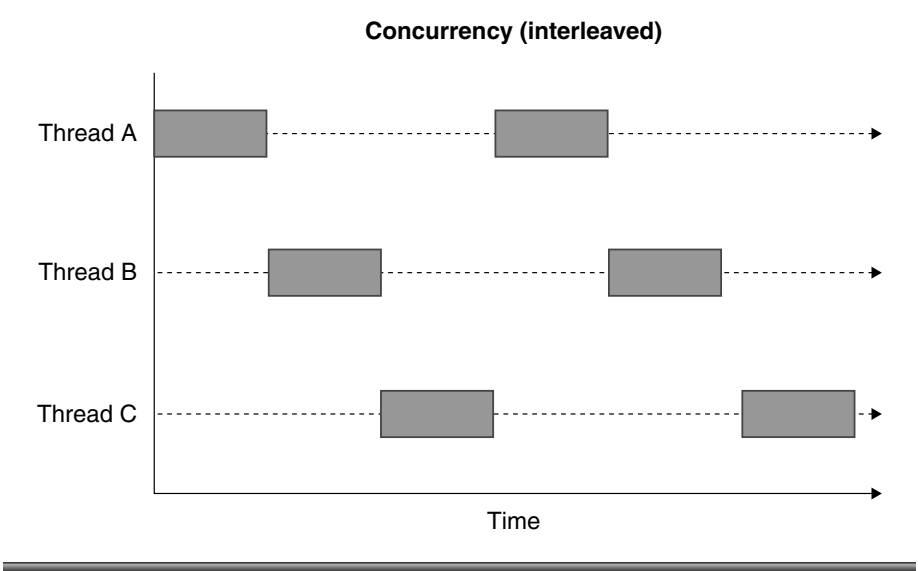
Figure 7.1 Concurrency interleaved
