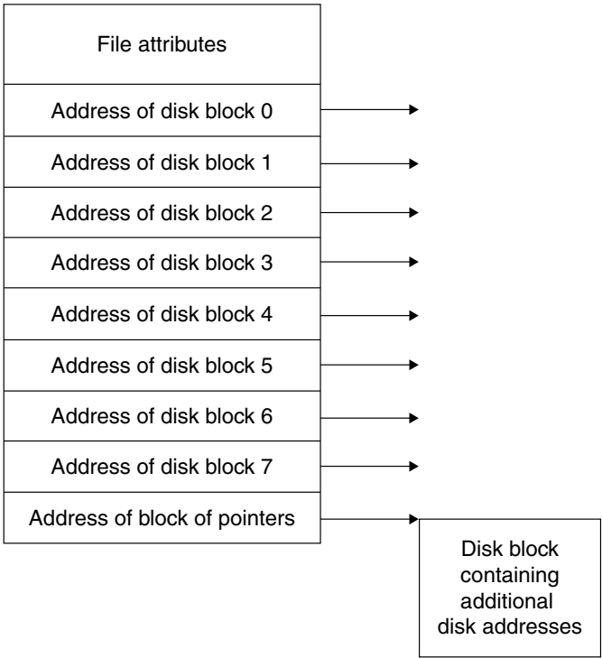
Figure 8.1 Sample i-node
